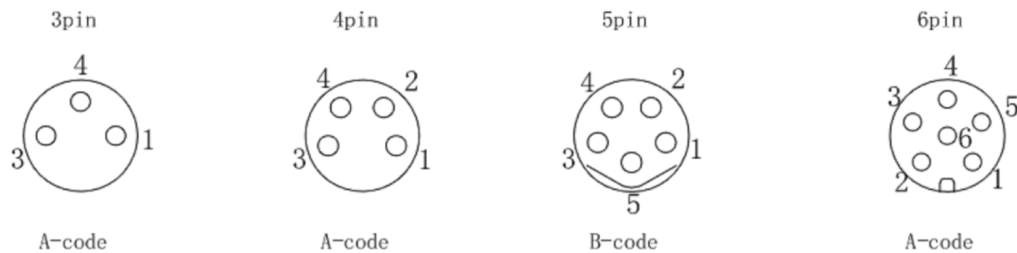
Pin assignment front view/针位分布前视图
